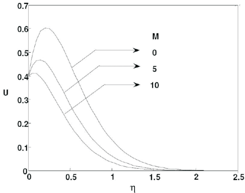
Figure 4: Velocity Profiles for different M
