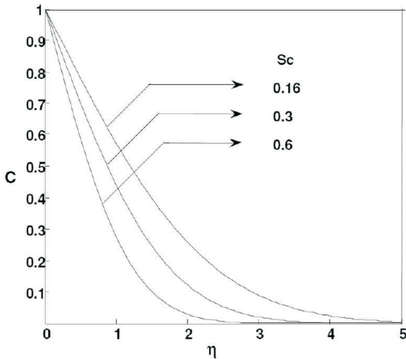
Figure 2: Concentration Profiles for different Sc
