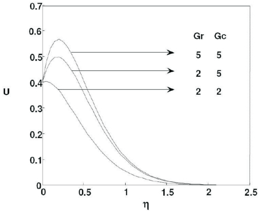
Figure 3: Velocity Profiles for different Gr and Gc
