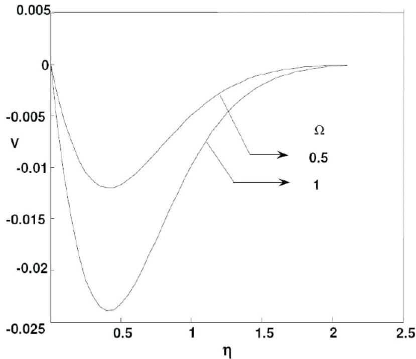
Figure 6: Secondary Velocity Profiles for different \Omega
