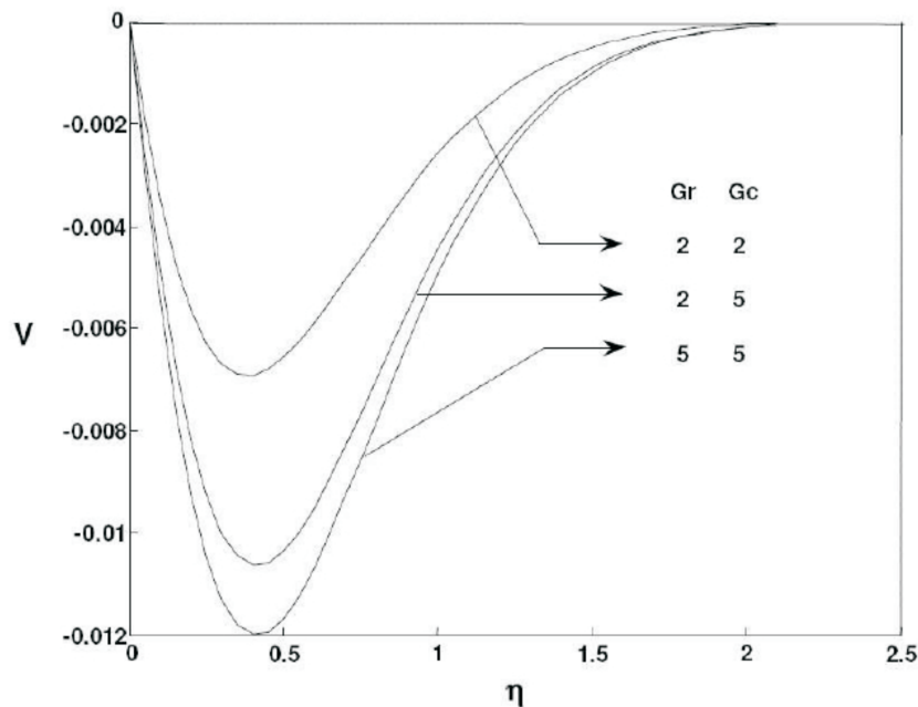
Figure 5: Secondary Velocity Profiles for different Gr and Gc
